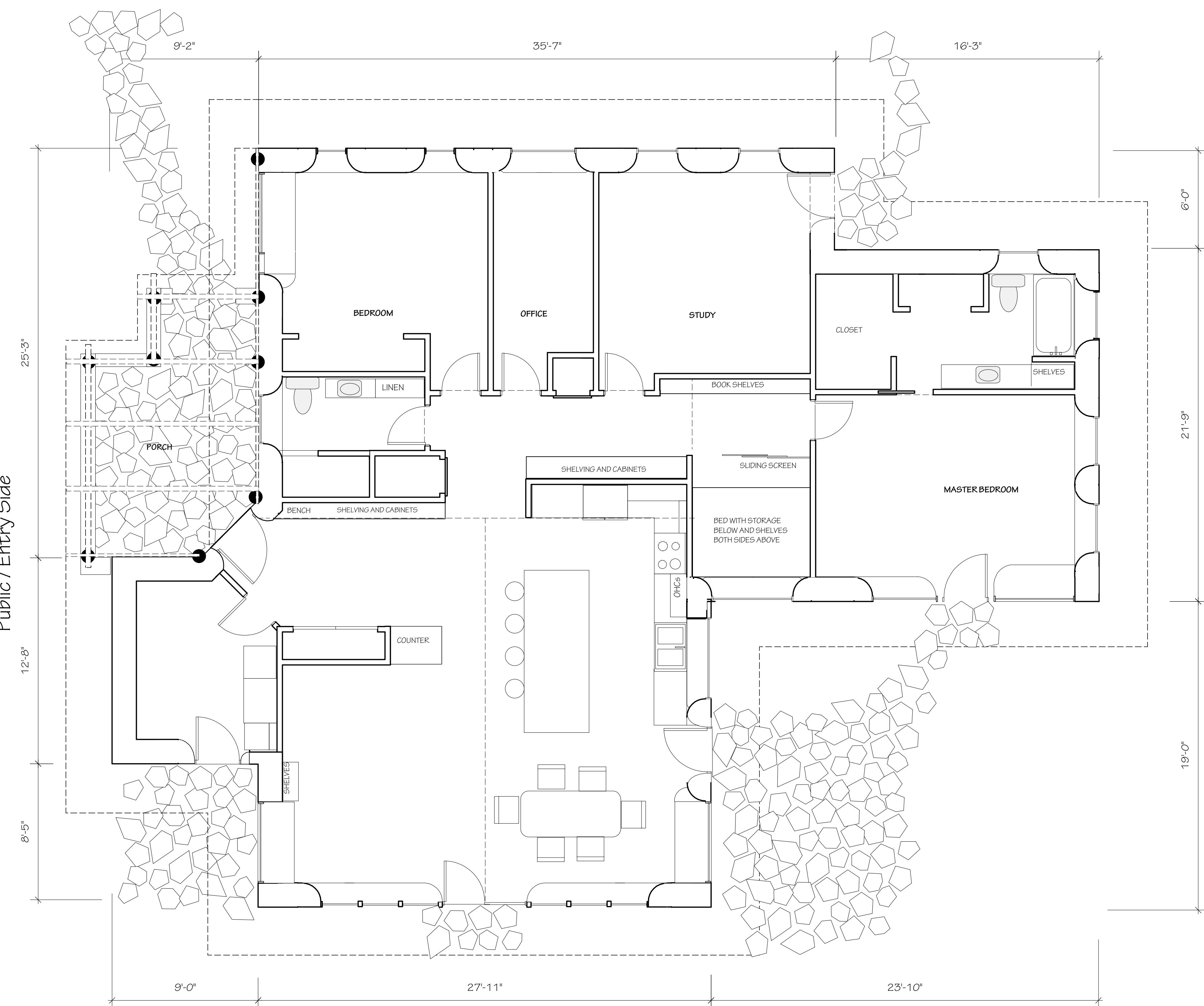
Floor Plan 1/4"=1'-0"
