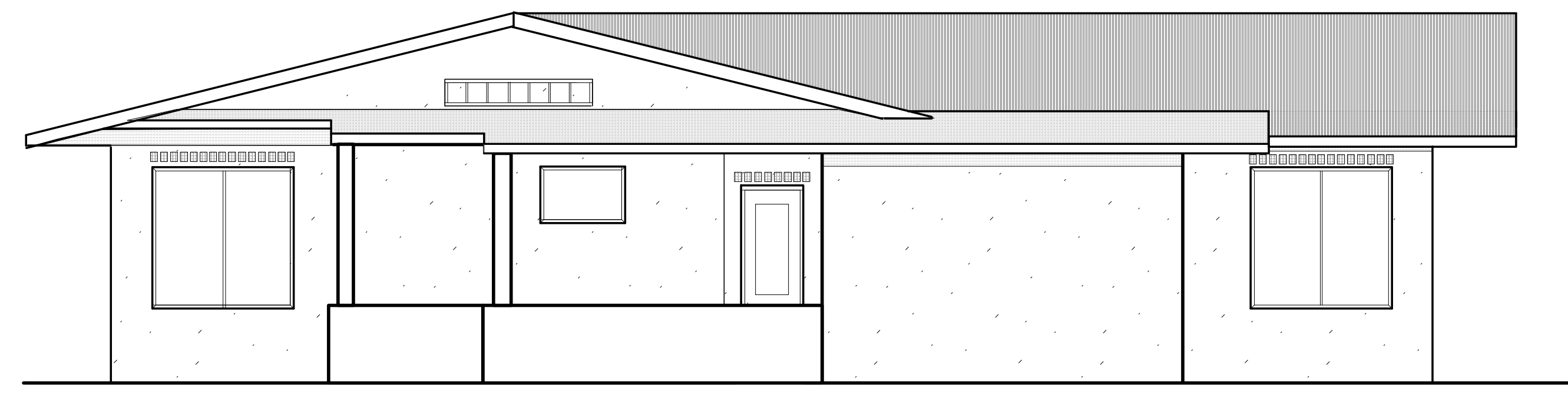
WEST ELEVATION 1/4"=1'-0"
