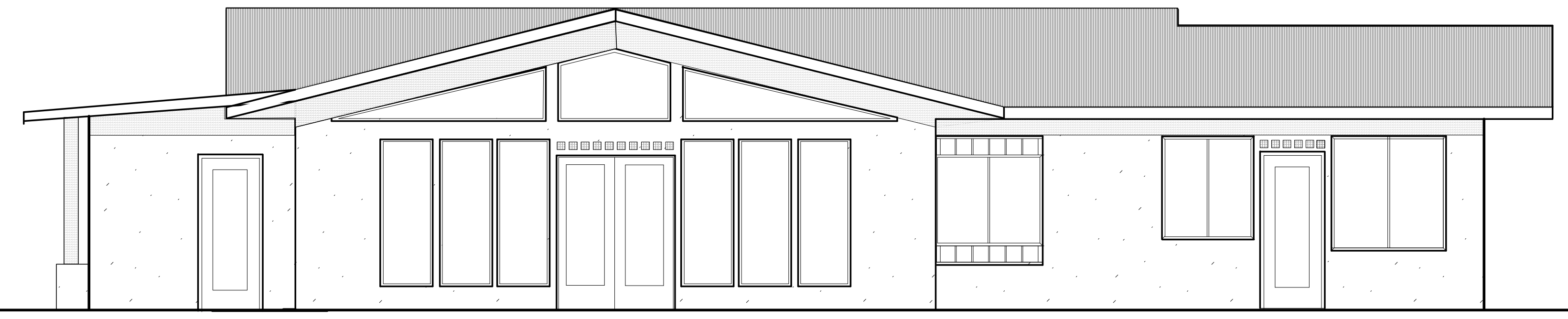
SOUTH ELEVATION 1/4"=1'-0"
