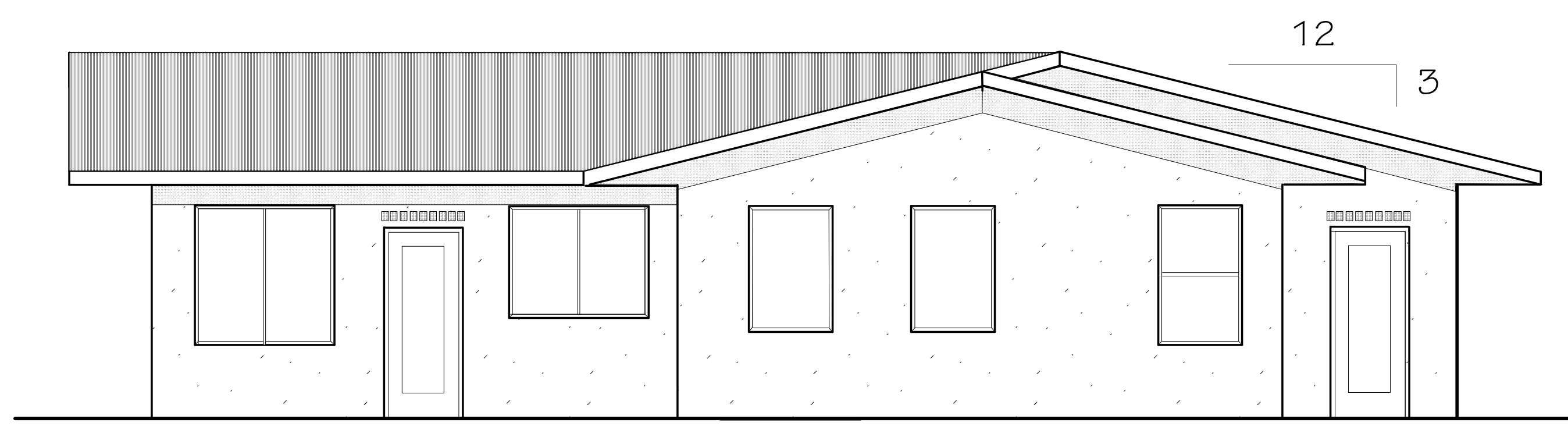
EAST ELEVATION 1/4"=1'-0"
